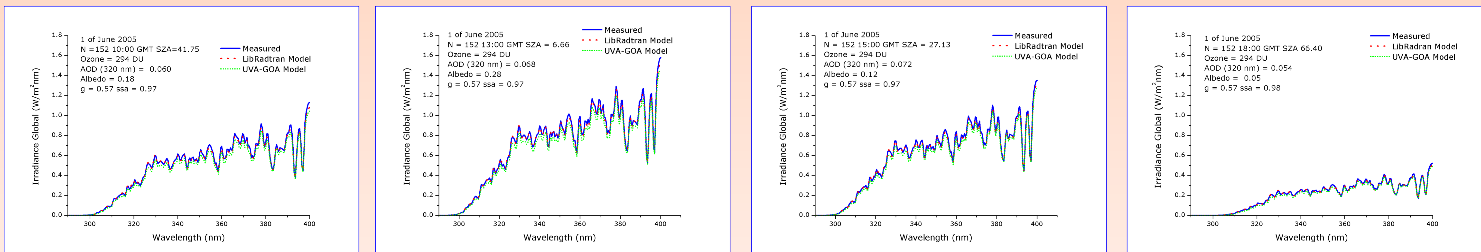
Figure 1.- Comparisons between the solar UV global irradiance spectra observed with spectroradiometer Bentham at Izaña in 1 June 2005, and simulated with the LibRadtran and UVA-GOA models at 4 different solar zenith angles.
