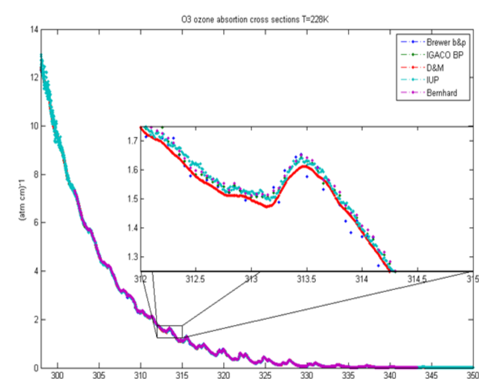
Figure 7: The five ozone cross section data sets at -45°C used on this work, Bass & Paur (Brewer), Bass & Paur (IGACO4), DBM Daumont, Malicet and Brion (IGACO4) the new set from Bremen university (IUP) and the set of B&P used by Bernhard 2005.
