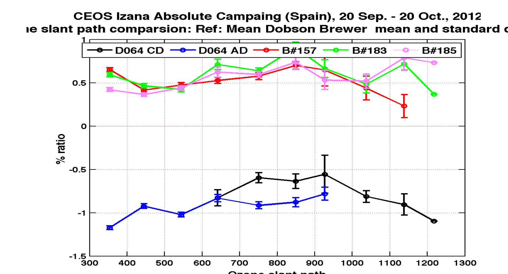
Figure 6: Ozone slant path (right) total ozone Brewer and Dobson t comparison during the campaign. The percentage ratio is represented: o_3-ref/ref with the reference the mean of the three brewer instruments and the Dobson AD/CD pairs.
