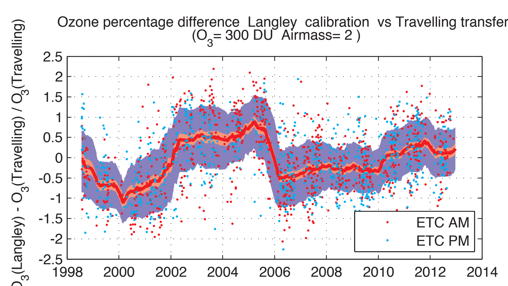
Figure 2: Effect on the Ozone measurement if we use the Langley calibration (Figure 1) vs the Calibration from travelling reference Brewer #017 on the RBCC-E primary reference Brewer #157 (Assuming an ozone total content of 300 DU and air mass = 2). The red line is the monthly smoothed percentage difference. The red area represent the 95% confidence interval of the mean and the blue area the standard deviation.
