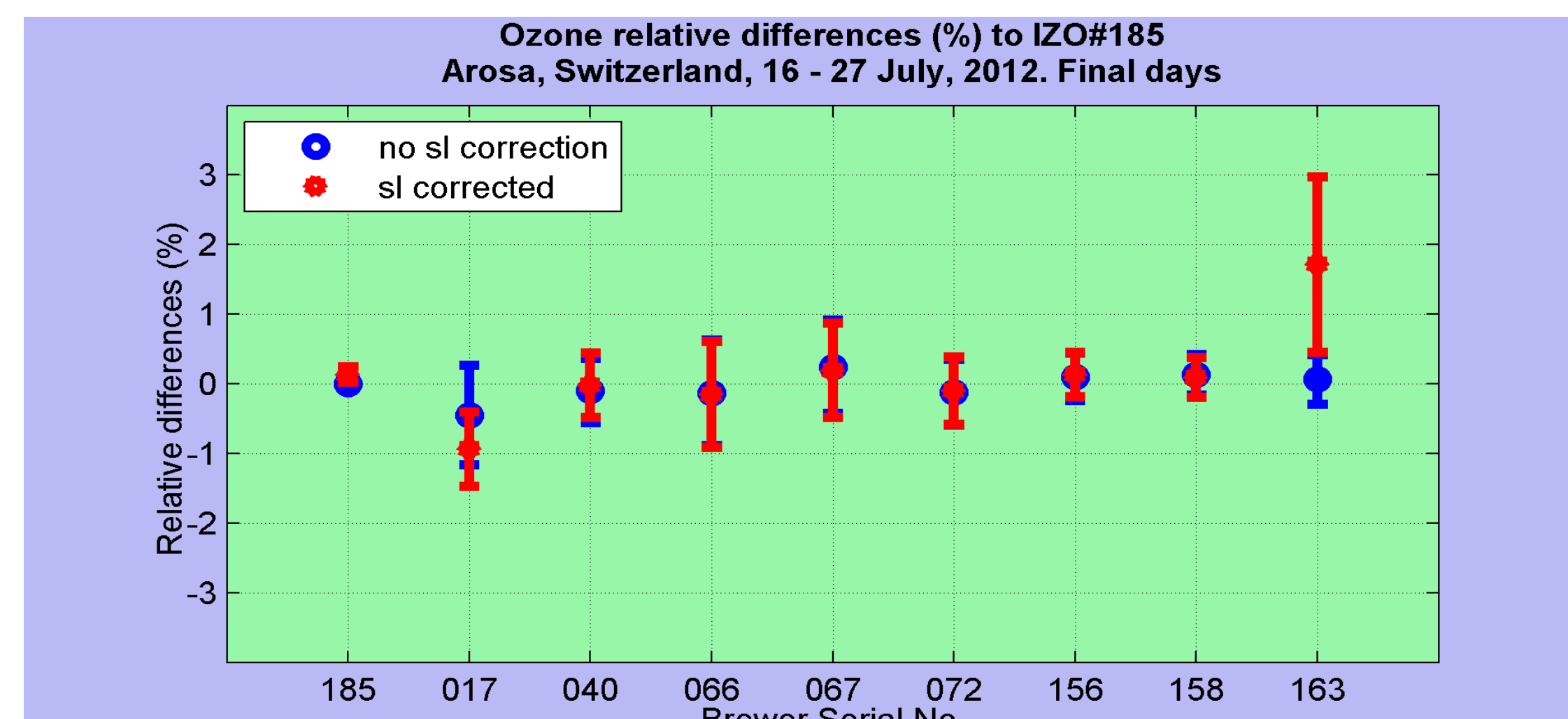
Figure 4: Ozone relative percentage differences of Arosa 2012 participating instruments to RBCC-E travelling standard Brewer #185. Ozone measurements collected during the final period are reprocessed using the final calibration constants.
