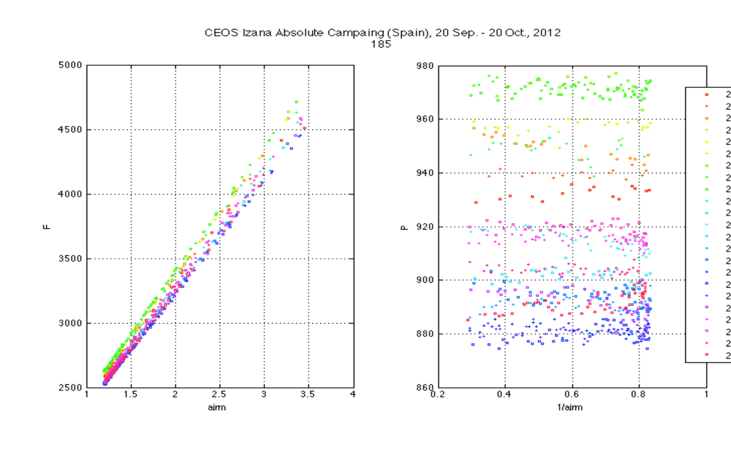
Figure 5: Langley plots for the Brewer 185 during the campaign. We show in the left panel the regression vs. \mu and in the right panel the Dobson method P = F-ETC/\nu vs. 1/\mu
