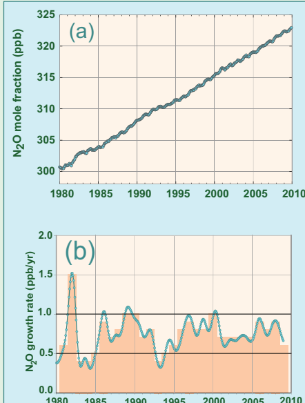
Figure 5. Globally averaged N 2 O mole fraction (a) and its growth rate (b) from 1980 to 2009. Annually averaged growth rate is shown by columns at (b).
