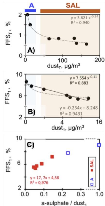
Figure 8.6. Fractional total Iron Solubility (FFST) versus total dust (A) and Fractional submicron Iron Solubility (FFS1) versus submicron dust (B) and versus the submicron ammonium-sulphate / dust ratio (C). Reproduced from Ravelo-Pérez et al. (2016). Samples collected in the Saharan Air Layer (SAL) and Atlantic westerly airflow (A) are differentiated)
