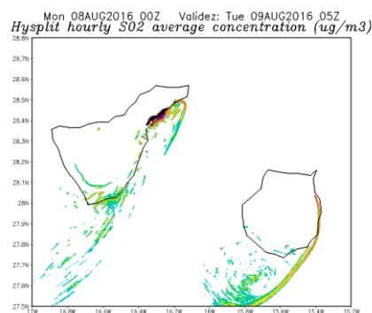
Figure 13.8. Average Hysplit SO 2 concentration shading contours forecasted on day 09/08/2016 at 05 UTC.
